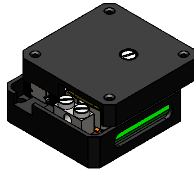
Right end stop +5 mm stroke
